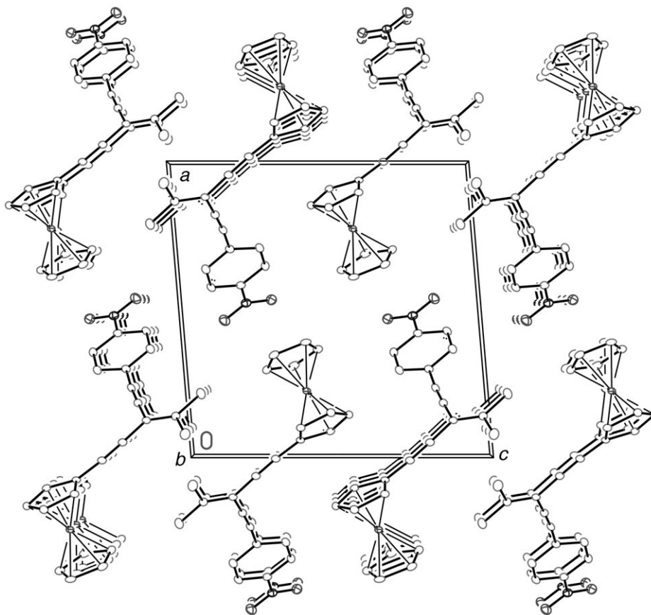
Fig. 5. Crystal packing of compound 8
