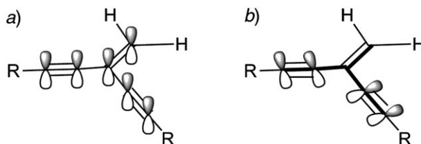
Fig. 6. Schematic illustration of orbitals in g-DEEs. a) Out-of-plane (vertical) p-orbitals (denoted \pi_{\perp} ), b) in-plane p-orbitals (denoted \pi_{\parallel} ) and \sigma -bonds (highlighted in bold, denoted \sigma_{\parallel} ).
